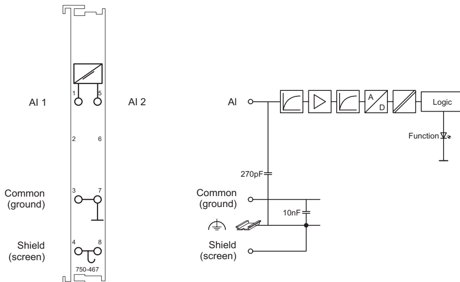
Fig. 2.1.1-3: 2-Channel Analog Input Module 750-467
